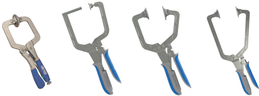
PREMIUM FACE CLAMP KHC-PREMIUM 3 1/4" REACH
